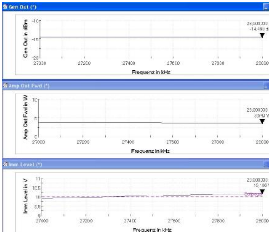
Common Mode (Calibration routine 10 V)
