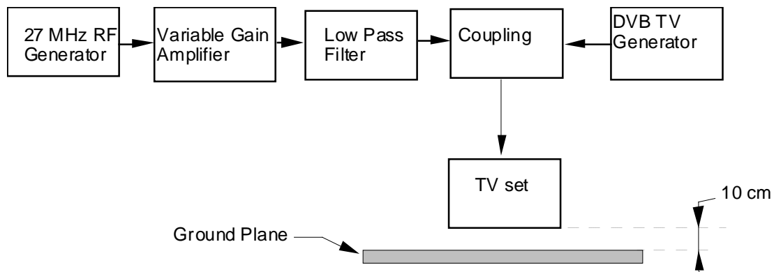
Figure A.3.1-1: Immunity test layout in laboratory
